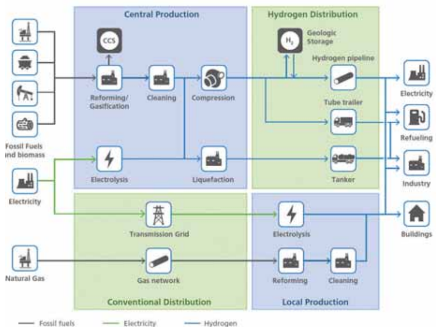
Figure 2: Hydrogen delivery pathways presented in the white paper: The Role of Hydrogen and Fuel Cells in Future Energy Systems
