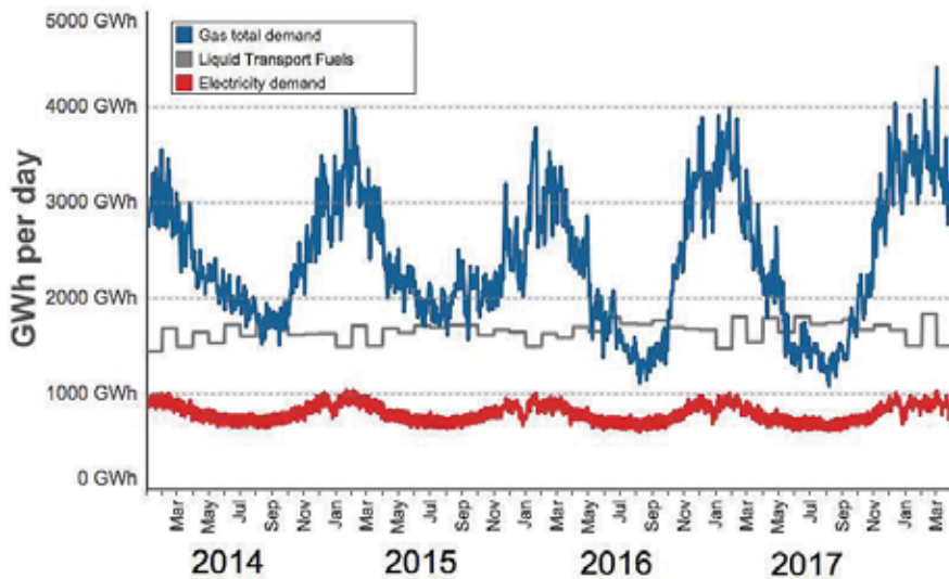
Figure 1: Demand for the major energy vectors in Britain, produced by Dr. Grant Wilson (University of Sheffield)
